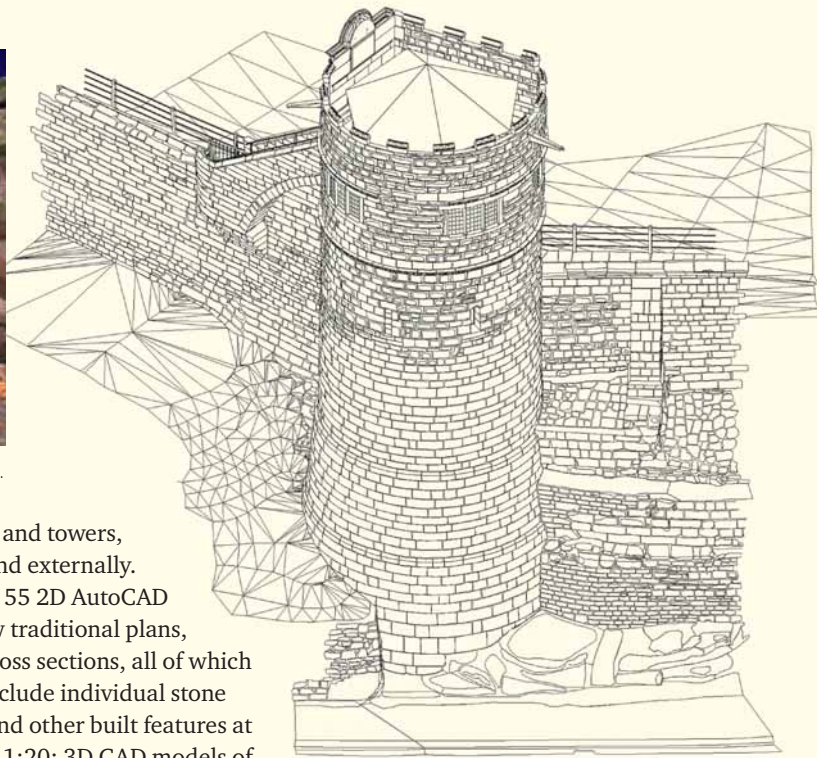
Fig CS12.3 AutoCAD 3D model with real-time hidden surfaces.
